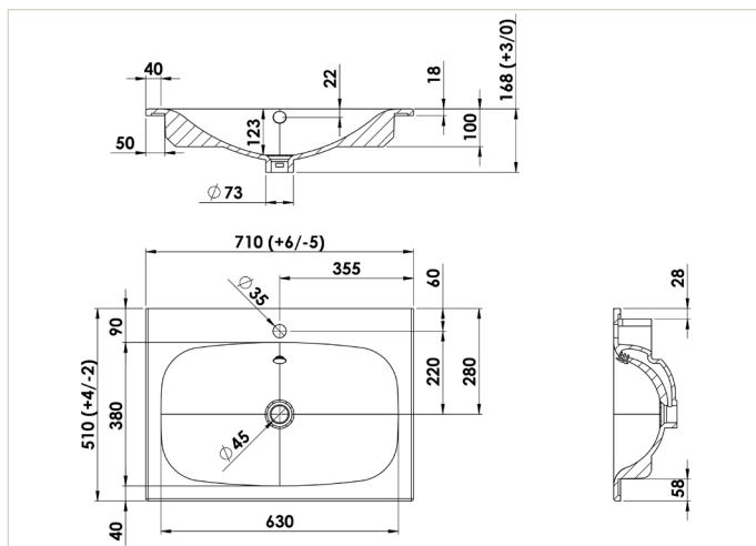
GOPLANC70CERB
