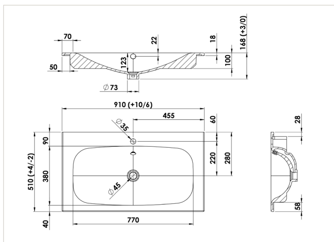
GOPLANC90CERB
