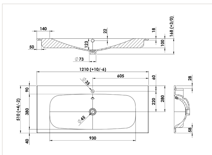
GOPLANC120CERB
