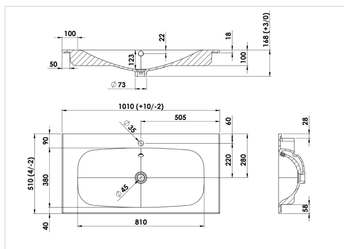
GOPLANC100CERB
