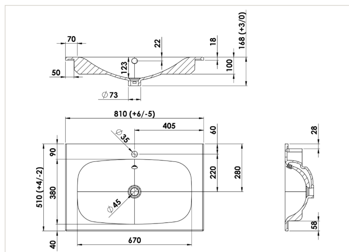
GOPLANC80CERB
