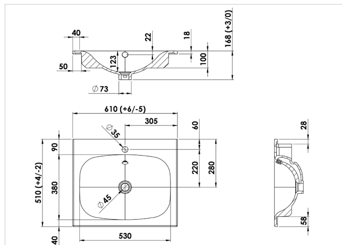
GOPLANC60CERB
