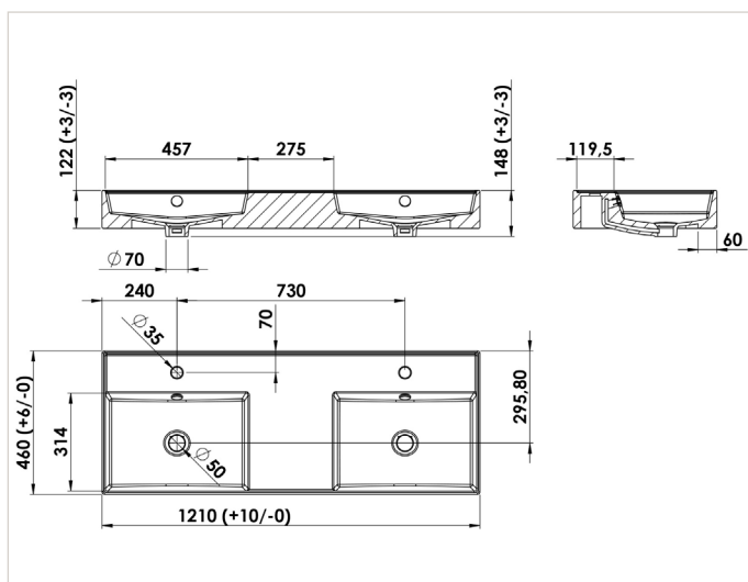
SEPLAN2120CERB
