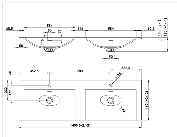
TEPLAN2140...
