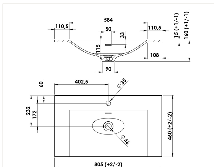
TEPLANC80...
