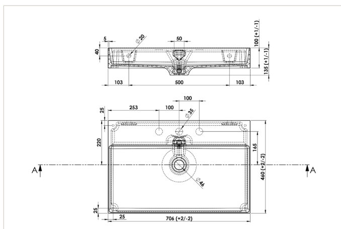
OGPLANC070...
