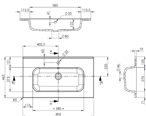
PRPLANC80BLB
