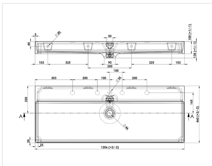
OGPLANC120...
