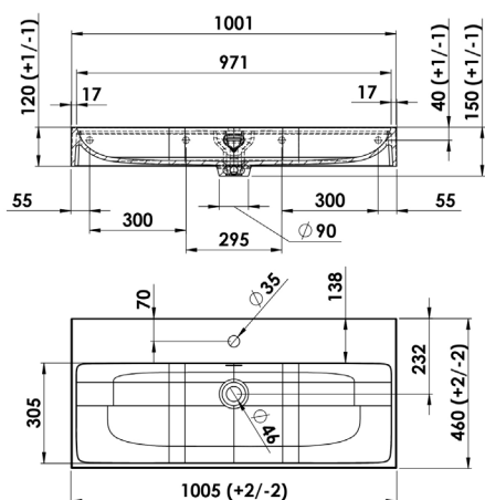
STPLANC100...
