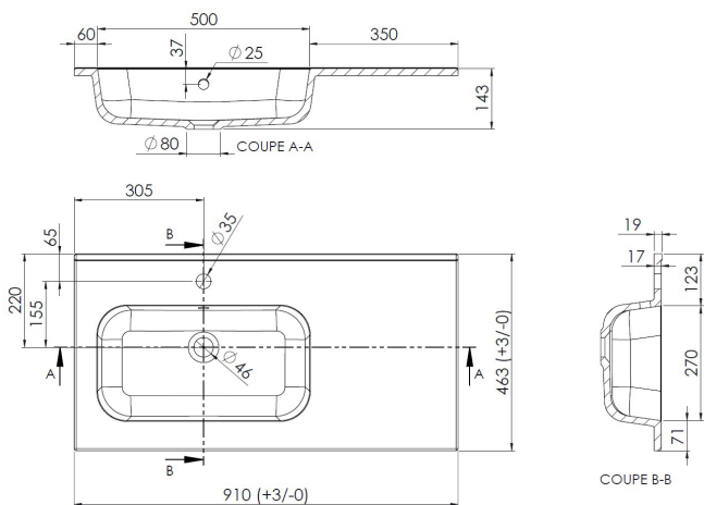
PRPLANG90BLB
