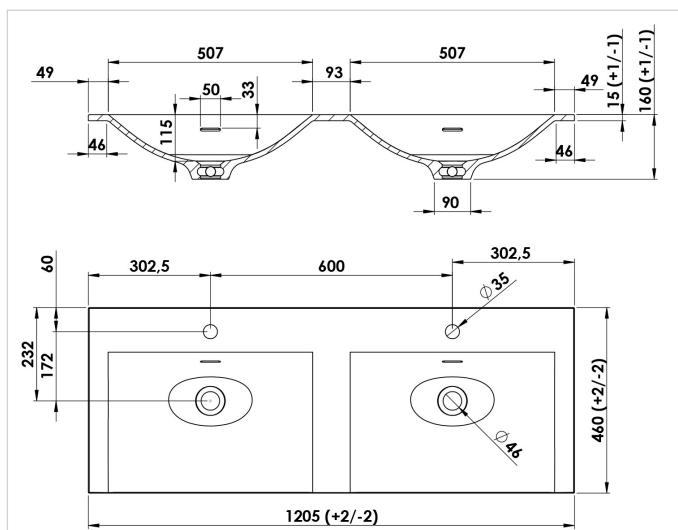
TEPLAN2120...
