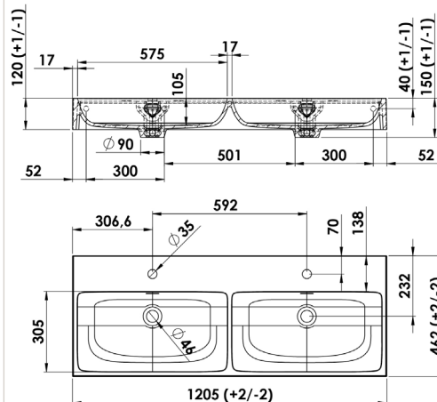
STPLAN2120...
