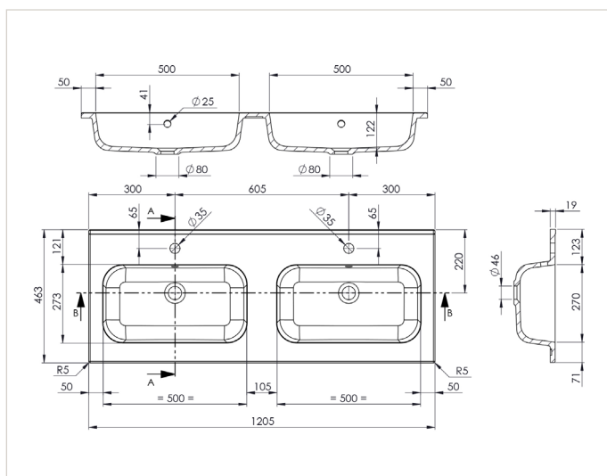
PRPLAN2120BLB double
