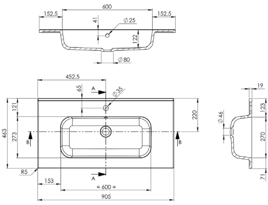
PRPLANC90BLB
