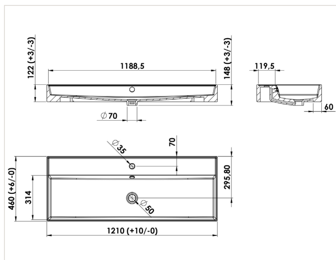
SEPLANC120CERB
