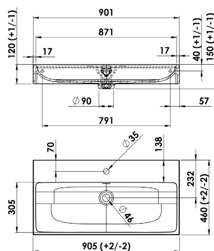
STPLANC090...
