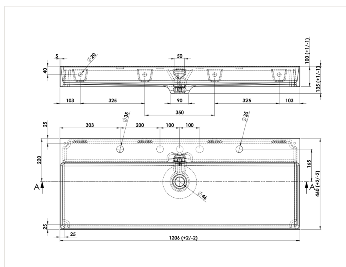
OGPLANM120...
